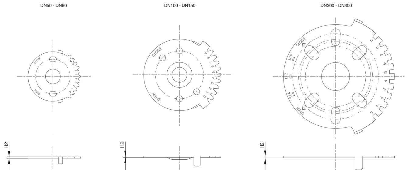
Figure 2. Notch plate
