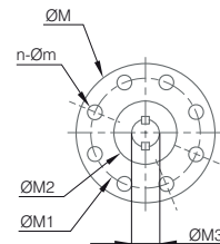
KEYWAY DN700 & DN800
