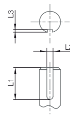
KEYWAY DN900 - DN1200
